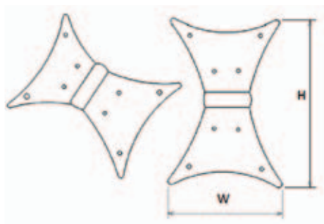
Butterfly hinge
