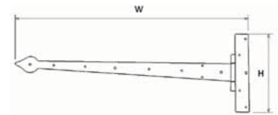
Arrow Head T hinge
