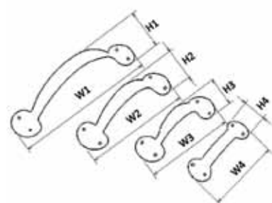
Bean Pull Handle - Beeswax
